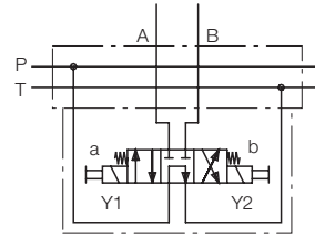
4/3 directional control valve with mounting plate for unpressurised cycles in central position. Ports A and B closed, not leakage-free.
