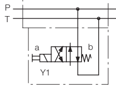
4/2 directional control valve with mounting plate for unpressurised cycles.
