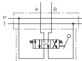
4/3 directional control valve with unpressurised cycle in central position, manually operated by lever, spring return. Ports A and B closed, not leakage-free.
