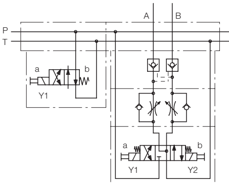
4/3 directional control valve with twin flow control valve and twin check valve. Ports A and B closed and leakage-free.
