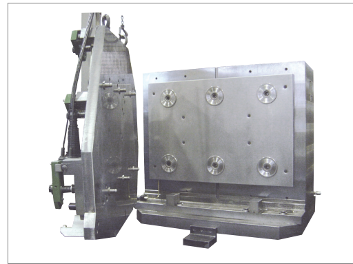
SPEEDY classic 1 fast closing clamp fitted to mounting tower with pipework, protected by cover plate
