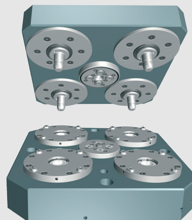
SPEEDY classic 1 TWISTER fast closing clamps, fitted in plate
