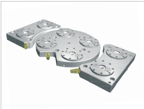
SPEEDY classic 1 fast closing clamps fitted in three separate plates, to increase the size of the working area on a 5-axis machine
