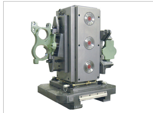
SPEEDY classic 1 fast closing clamp fitted to each side of the mounting tower with pipework, protected by cover plate
