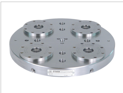
SPEEDY classic 1 fast closing clamps fitted in round plate, hydraulic connection via rotary joint
