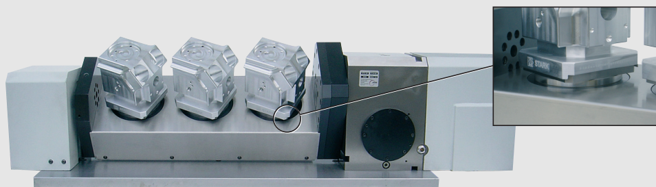
Square SPEEDY classic 1 STANDARD for single mounting (positioned secured against turning)
