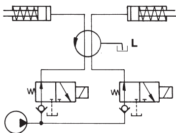
Hydraulic circuit diagram (Example)
