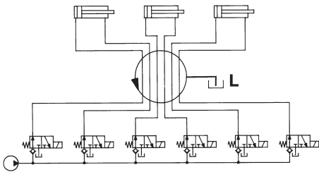
Hydraulic circuit diagram (Example)
