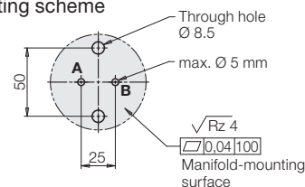
Connecting scheme
