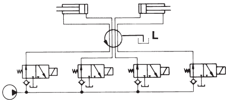
Hydraulic circuit diagram (Example)
