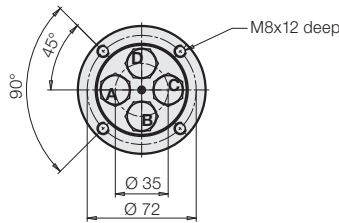
Connecting scheme
