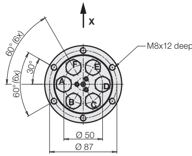
View X
