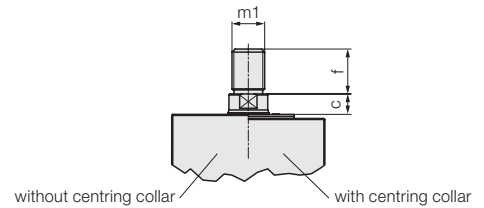
Centring collar only with housing RB and RC
